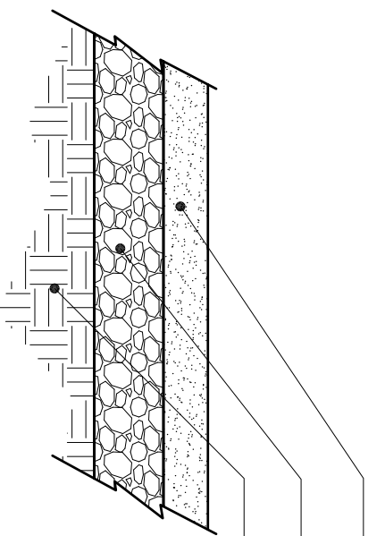
A HIGH TRAFFIC AREAS DECOMPOSED GRANITE WITH AGGREGATE BASE
