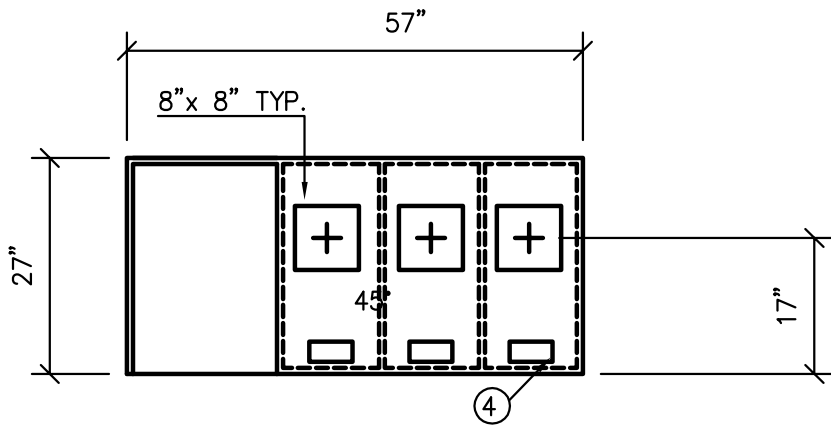
SMALL CABINET TOP VIEW
