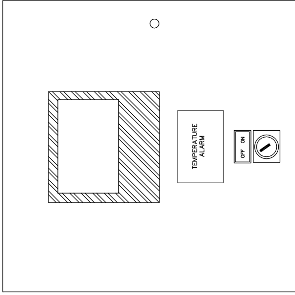
FRONT_PANEL_LAYOUT
