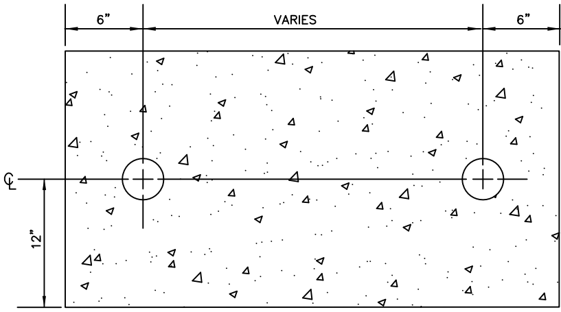
TOP VIEW OF SLAB
